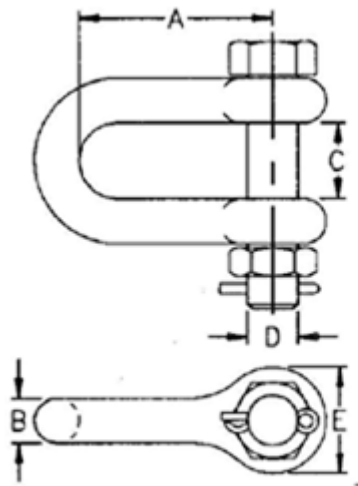
Bolt, Nut and Cotter Key (BNC)
