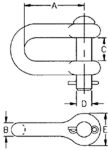
Pin and Cotter Key
